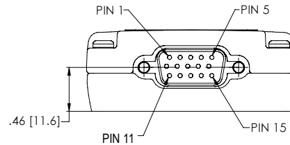
Male D-sub connector
