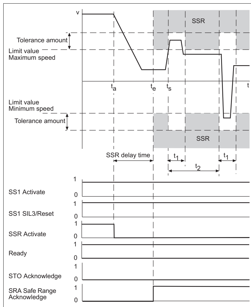
▶ Tolerance amount as % of the two limit values, maximum and minimum speed ▶ t_a : Activation of safety function SSR ▶ t_e : Once the SSR delay time has elapsed, the speed is monitored ▶ t_s : Speed v exceeds the limit value and activates the tolerance range (tolerance amount, tolerance time, tolerance period) ▶ t_1 : Tolerance time ▶ t_2 : Tolerance period ▶ SS1 Activate: Input for safety function SS1 ▶ SS1 SIL3/Reset: Input for SIL 3 and reset ▶ SSR Activate: Input for safety function SSR ▶ Ready: Output for operating status of safety card and second output for feedback from safety function STO
