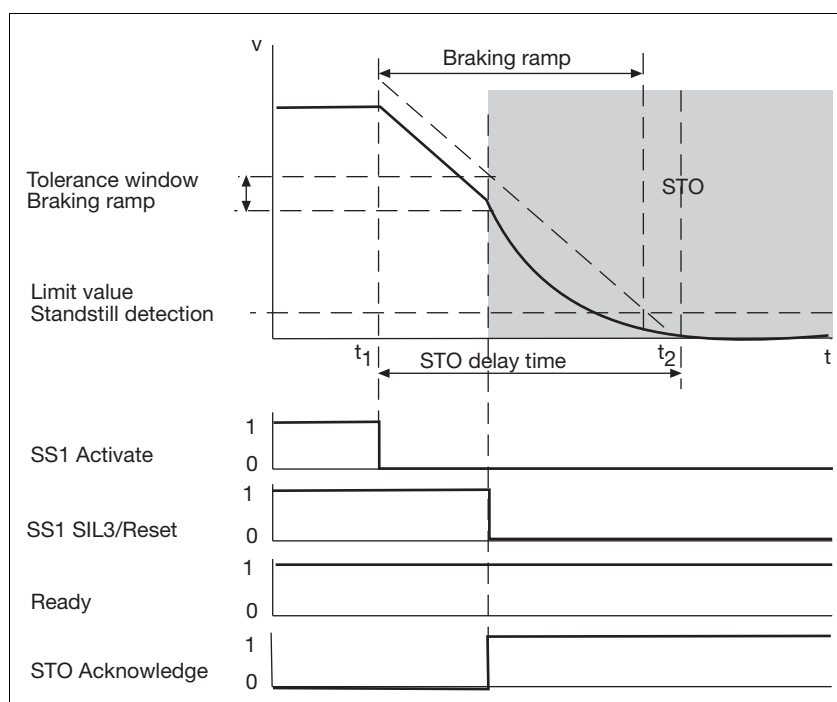
Fig. 4-4: Safety function SS1
