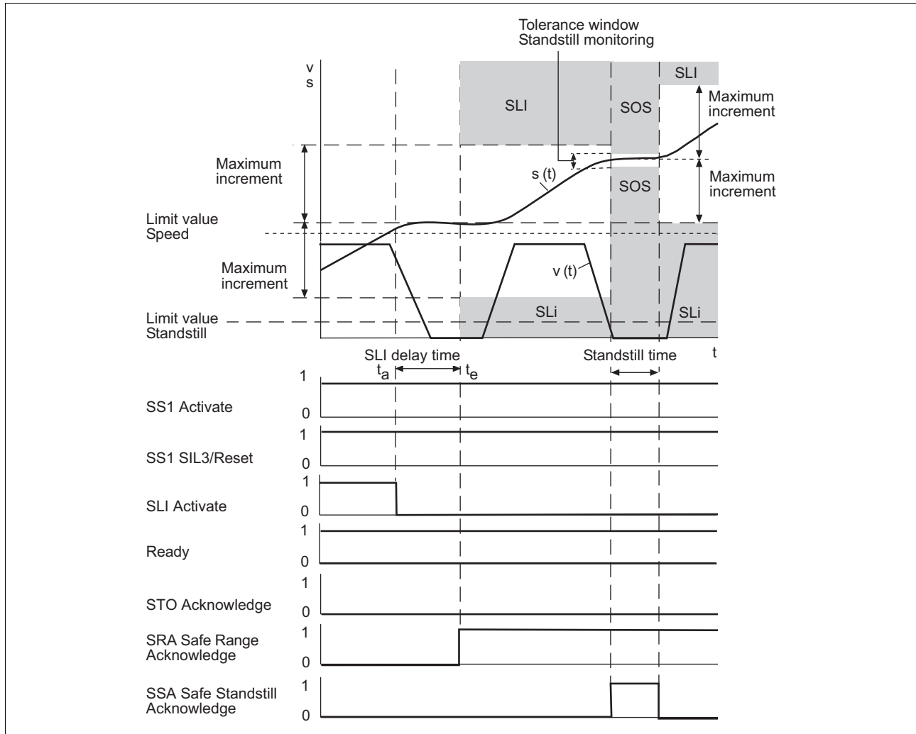
Fig. 4-15: Safety function SLI with automatic activation
