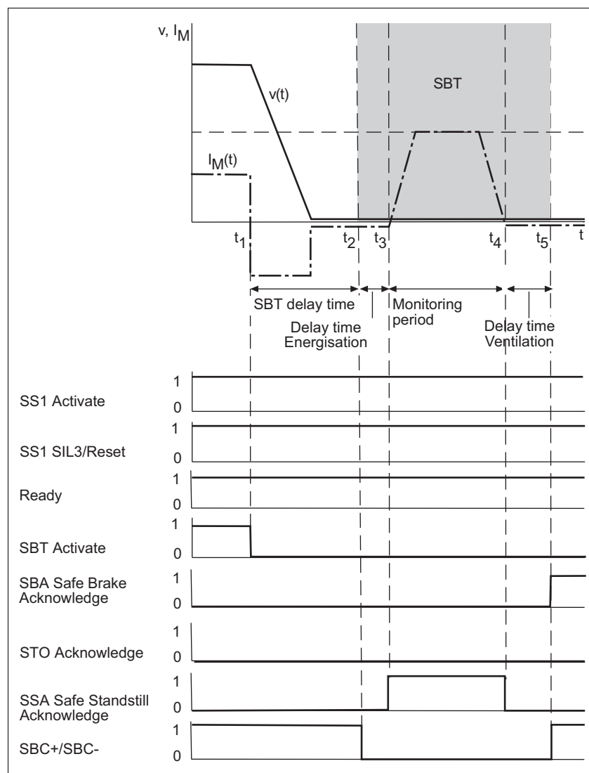
Fig. 4-18: Safety function SBT
