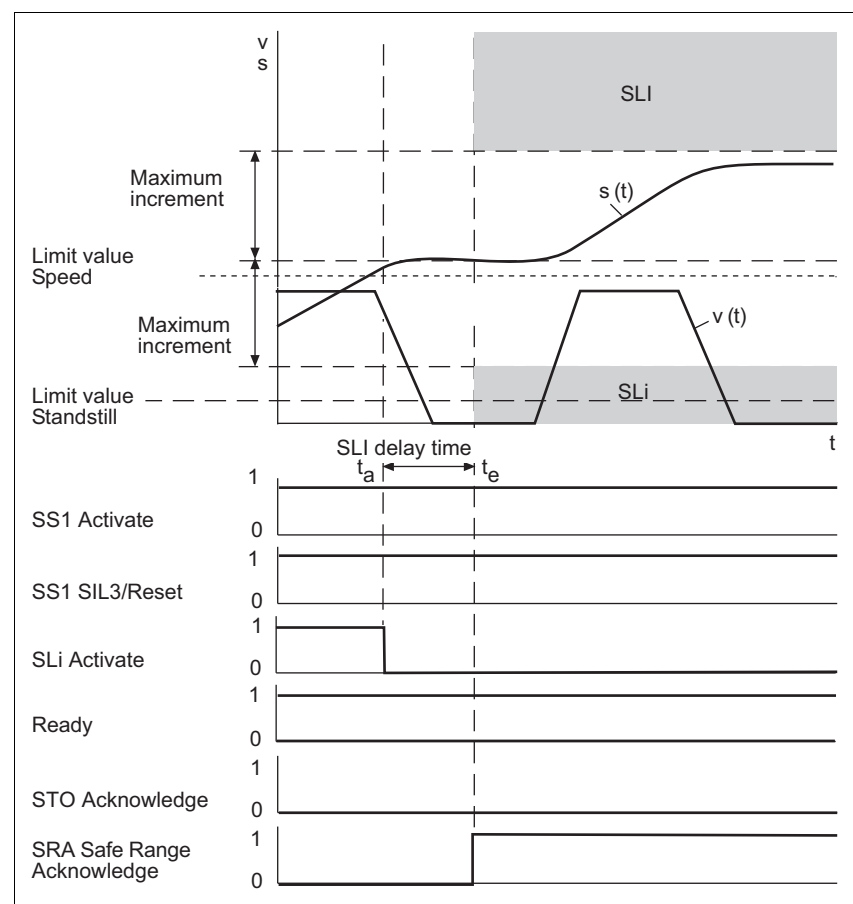
Fig. 4-14: Safety function SLI without automatic activation
